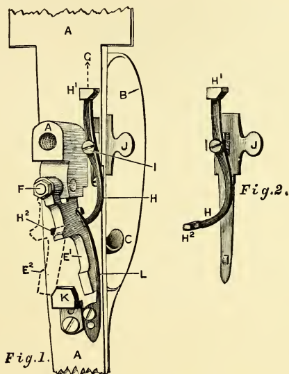
Charles Lancaster's Single-trigger Mechanism for Double-barrel Gun.
